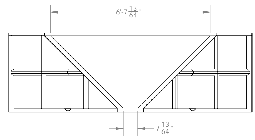
END VIEW (LOOKING UP STREAM)
