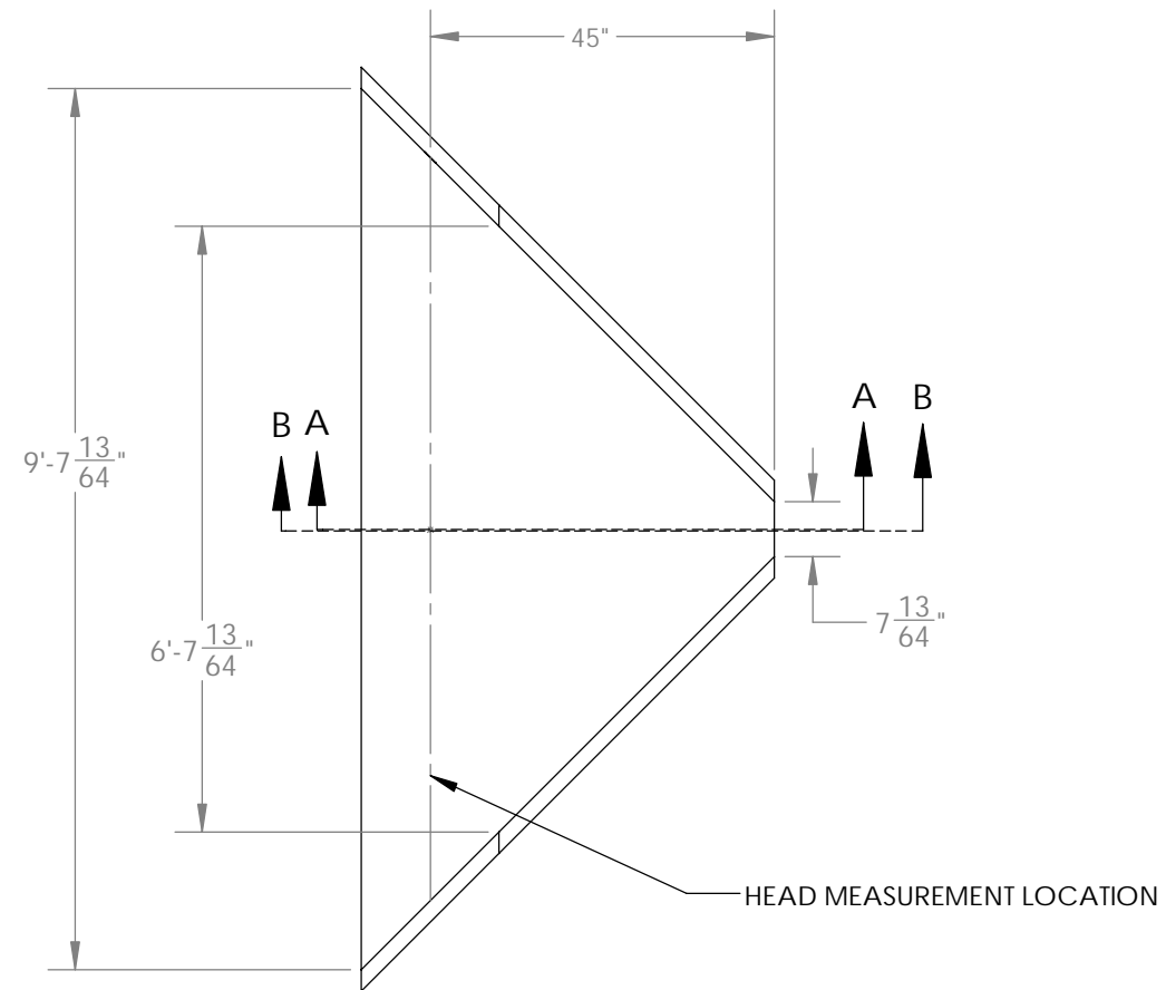
PLAN VIEW (SPREADER BARS REMOVED FOR CLARITY)
