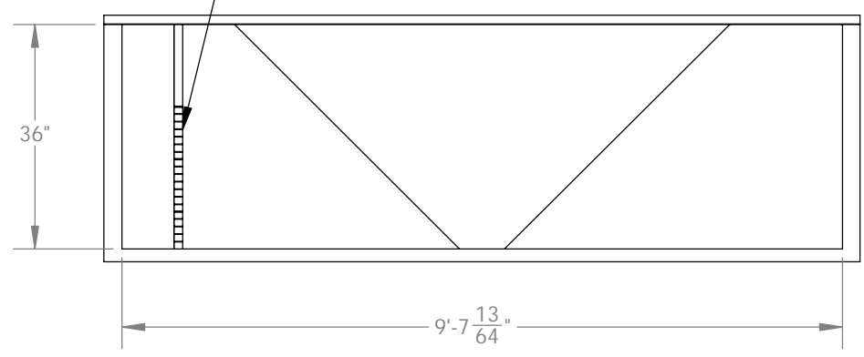
END VIEW (LOOKING DOWN STREAM)
