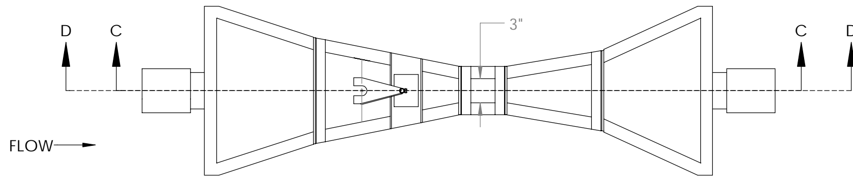
PLAN VIEW
