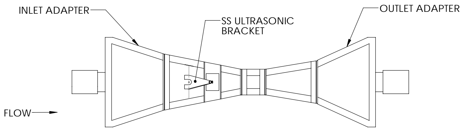
PLAN VIEW
