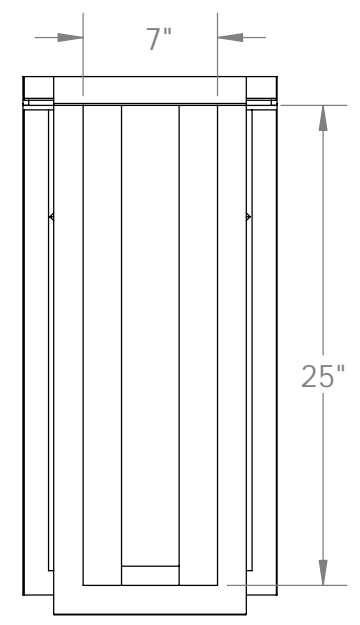
END VIEW (LOOKING UPSTREAM)
