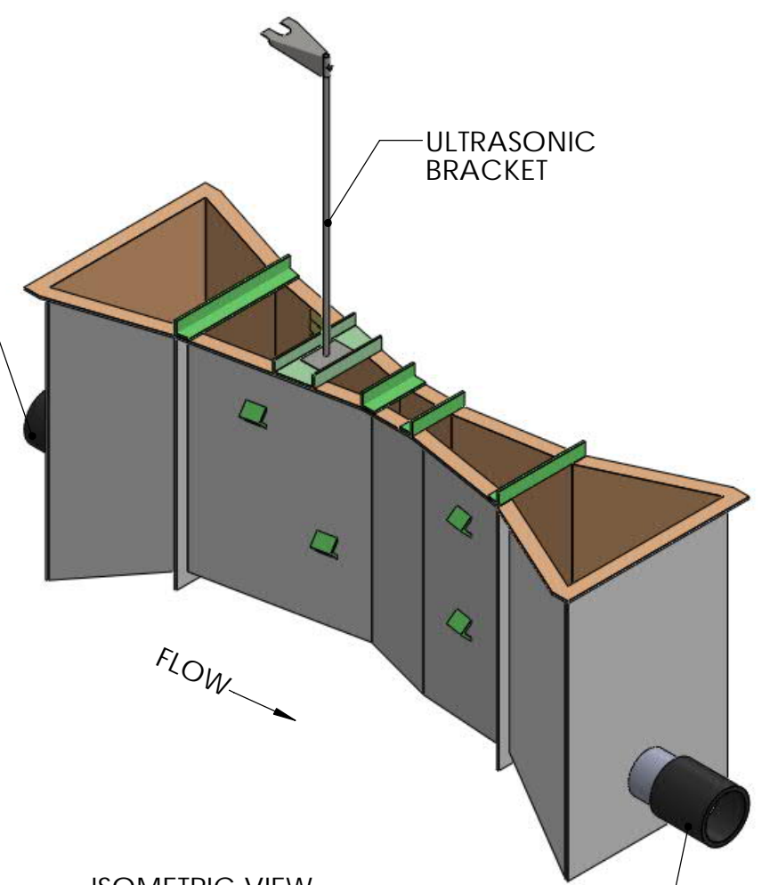
ISOMETRIC VIEW
