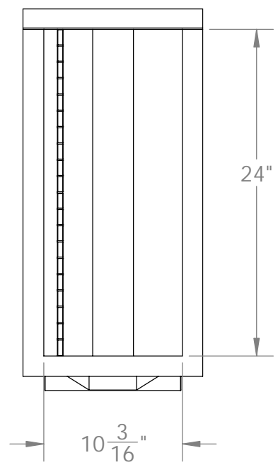
END VIEW (LOOKING DOWNSTREAM)
