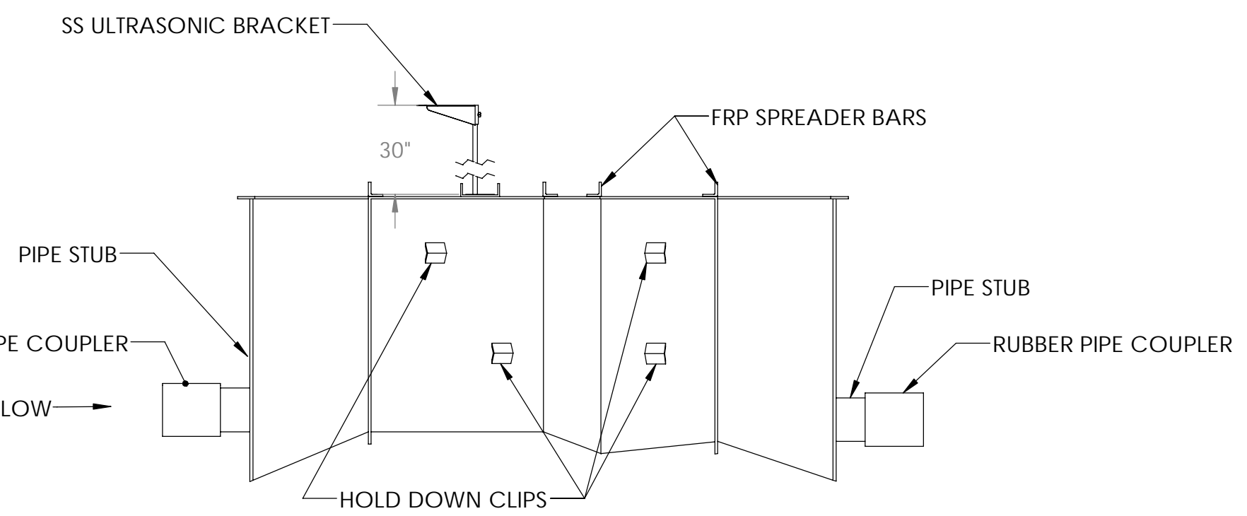
SIDE VIEW
