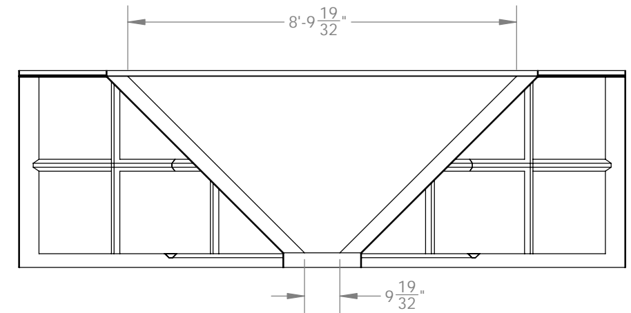
END VIEW (LOOKING UP STREAM)
