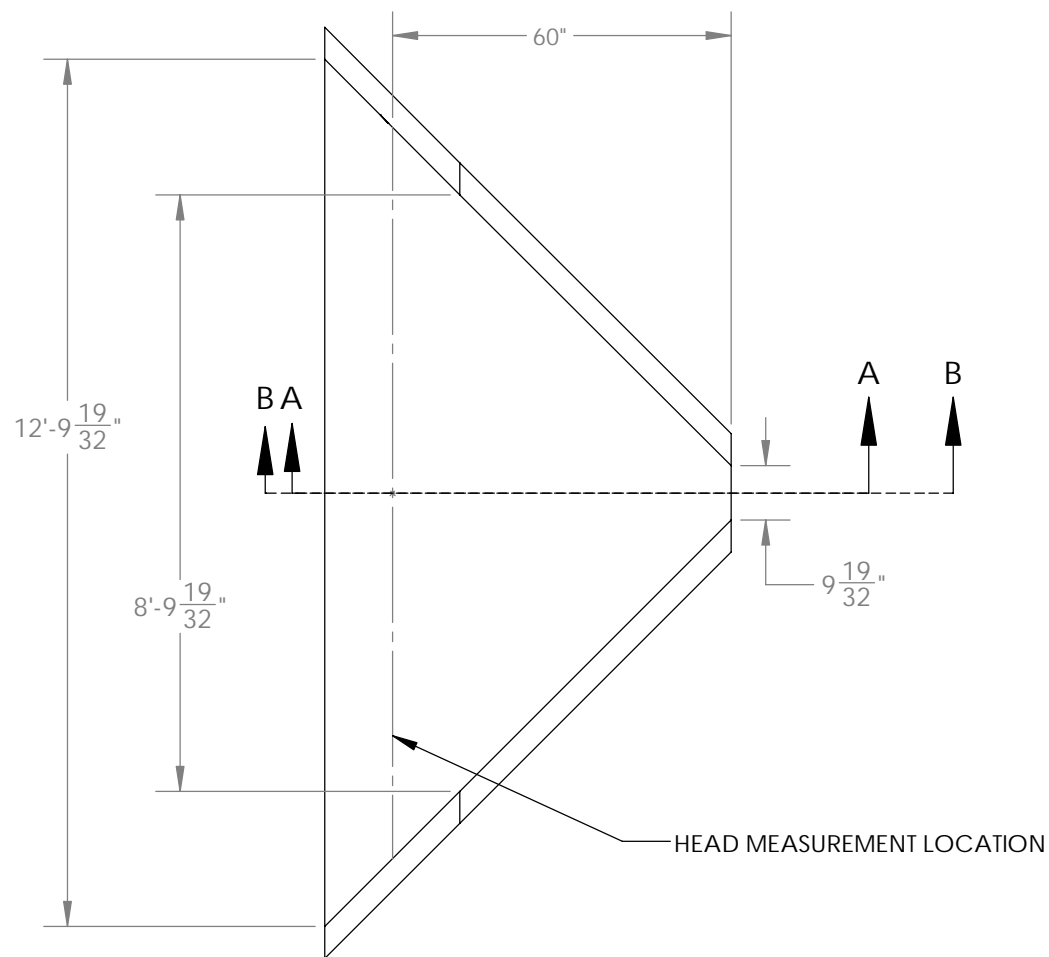
PLAN VIEW (SPREADER BARS REMOVED FOR CLARITY)
