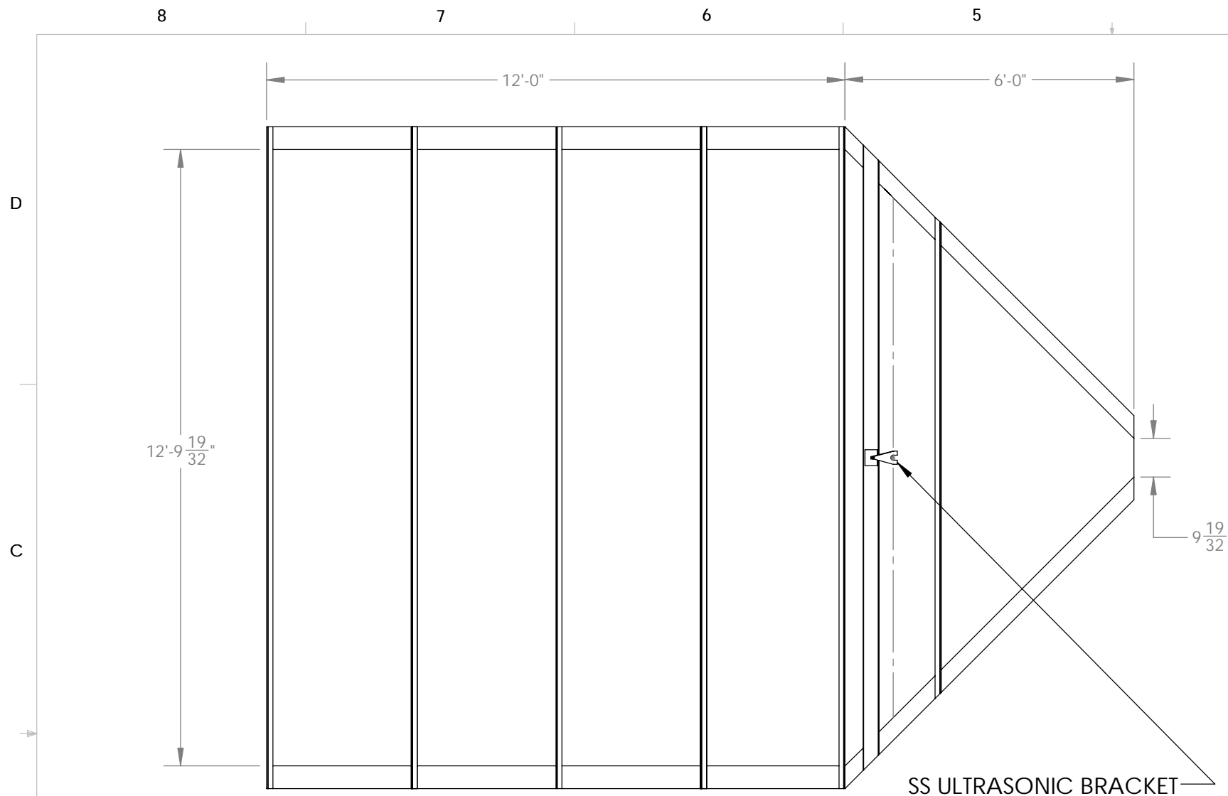
PLAN VIEW
