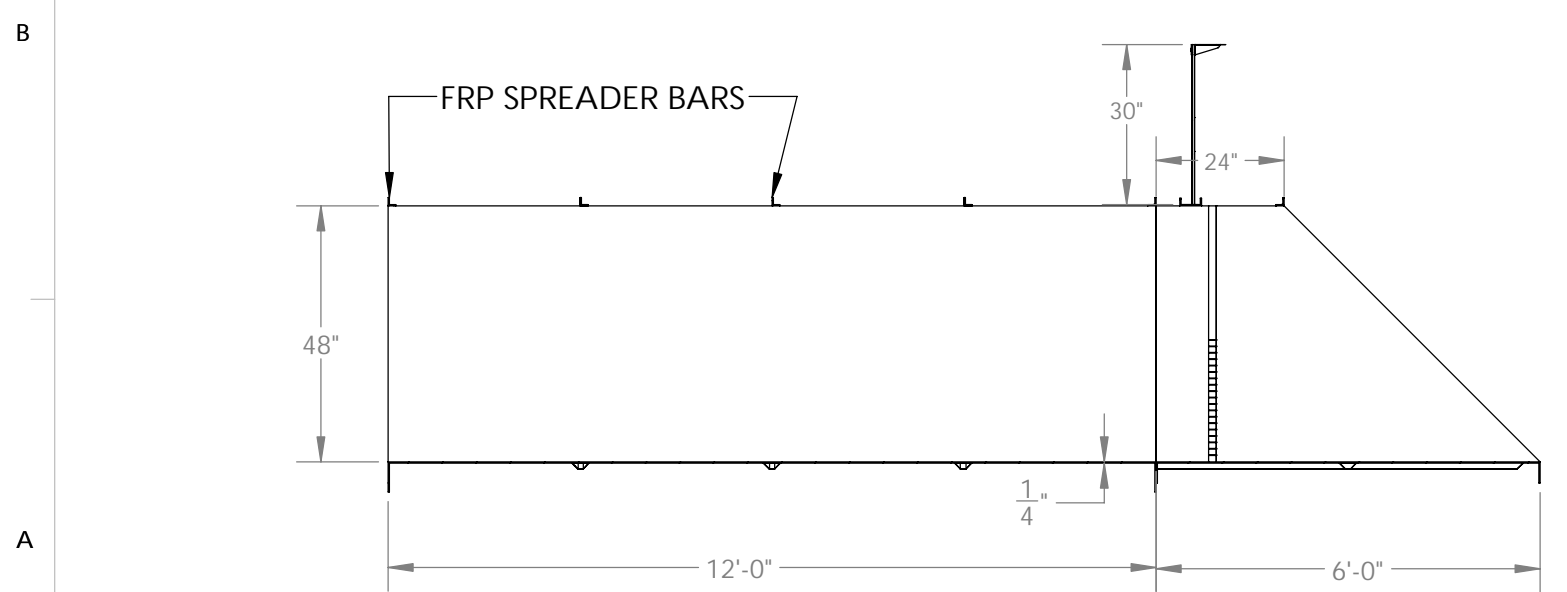
SECTION C-C
