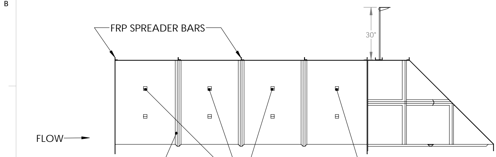
PLAN VIEW
