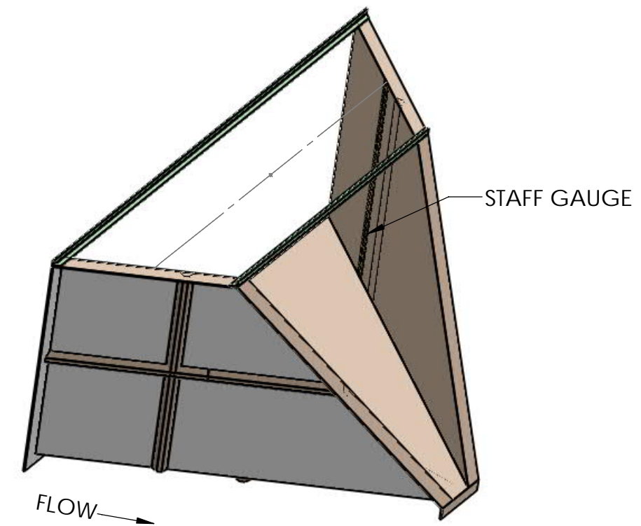
ISOMETRIC VIEW
